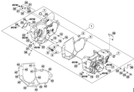
TAV.01 Carter completo - Crankcase, assy - Carter complet - Kurbelwellengehäuse, KPL - Carter completo
